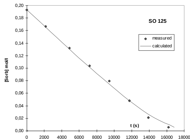
Fig. 6 Hydrogenation of sorbic acid, 44 mL bmim PF 6 , 60 mL MTBE, 30 mL dibutyl ether, 25 mmol sorbic acid, 16 bar H 2 , experiment SO 125; [cat] = 4.90 \times 10^{-4} mol/l; T = 30^\circ\text{C} ; k_2 [H_2]_0 = 0.0285 1/s; K_m = 0.014 mol/l
