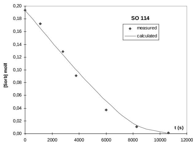
Fig. 5 Hydrogenation of sorbic acid, 44 mL bmim PF 6 , 60 mL MTBE, 30 mL dibutyl ether, 25 mmol sorbic acid, 16 bar H 2 , experiment SO 114; [cat] = 6.15 \times 10^{-4} mol/l; T = 34^\circ\text{C} ; k_2 [H_2]_0 = 0.0462 1/s; K_m = 0.021 mol/l
