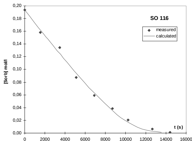
Fig. 4 Hydrogenation of sorbic acid, 44 mL bmim PF 6 , 60 mL dibutyl ether, 25 mmol sorbic acid, 16 bar H 2 ; concentration-time-diagram; [cat] = 4.83 \times 10^{-4} mol/l; T = 34^\circ\text{C} ; k_2 [H_2]_0 = 0.0462 1/s; K_m = 0.021 mol/l
