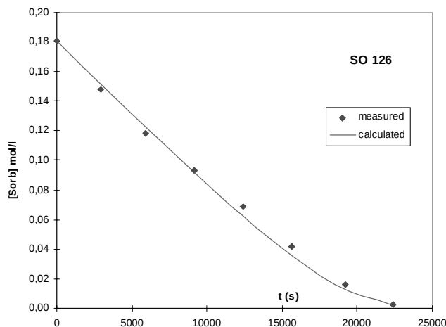
Fig. 7 Hydrogenation of sorbic acid, 44 mL bmim PF 6 , 60 mL MTBE, 30 mL dibutyl ether, 25 mmol sorbic acid, 16 bar H 2 , experiment SO 126; [cat] = 3.77 \times 10^{-4} mol/l; T = 30^\circ\text{C} ; k_2 [H_2]_0 = 0.0285 1/s; K_m = 0.014 mol/l
